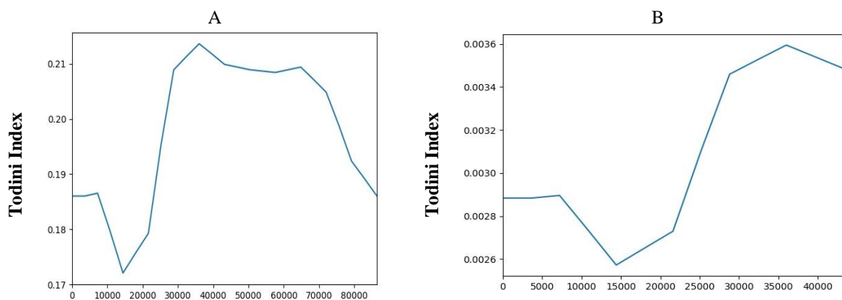
Fig. 12- Todini index for Scenario 12 A) before the earthquake B) after the earthquake
