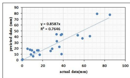
Fig.1- Comparison of the actual and predicted data by AA
