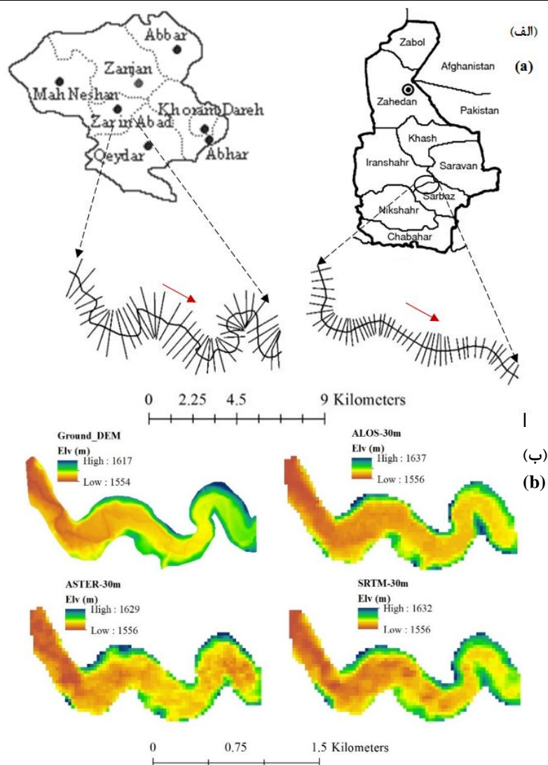
Fig. 1- a) Layout map of the study areas and b) DEMs used in SojasRood river, based on different DEM sources
