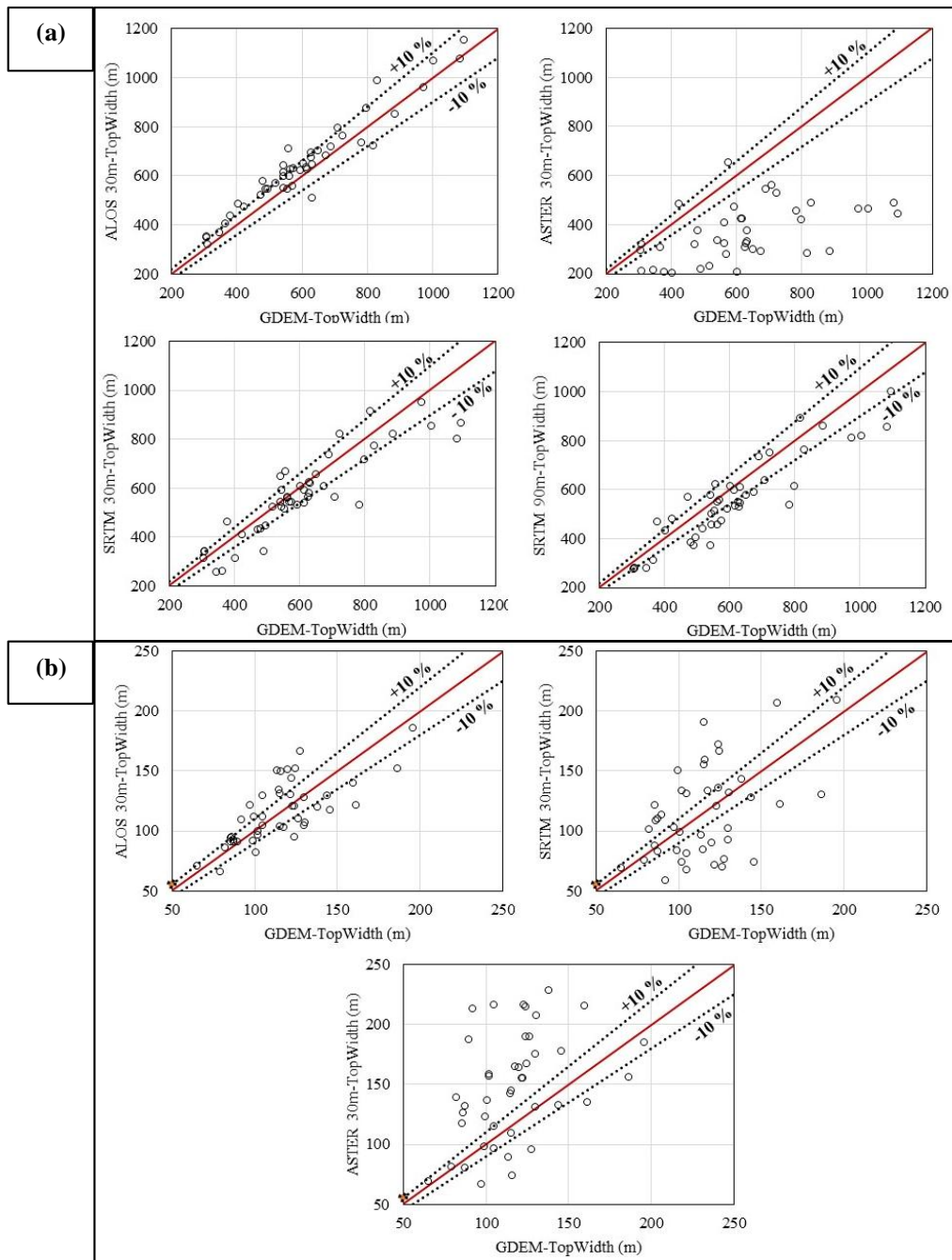
Fig. 6- Comparison of different DEM sources and topographic map in simulating inundated extent, (a) Sarbaz river; and (b) SojasRoad river
