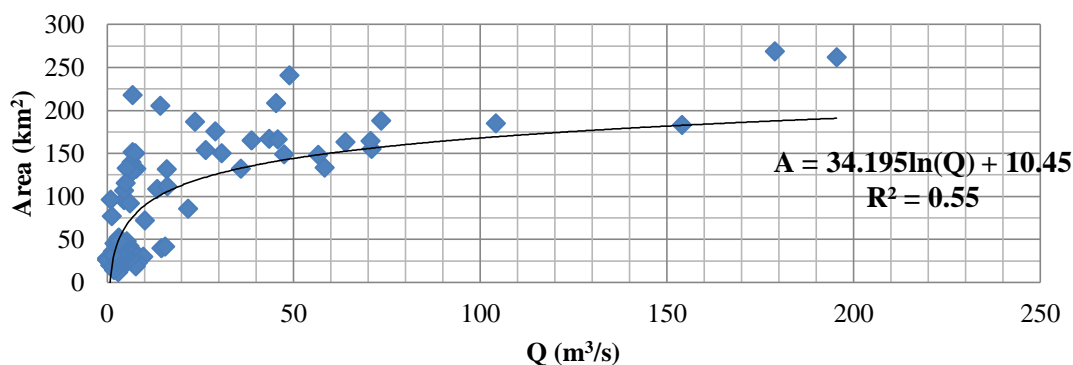
Fig. 12- Relationship between the area of flood plain and input discharge for southern area of Urmia Lake
