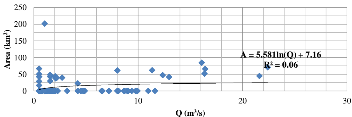
Fig. 13- Relationship between the area of flood plain and input discharge for south eastern area of Urmia Lake
