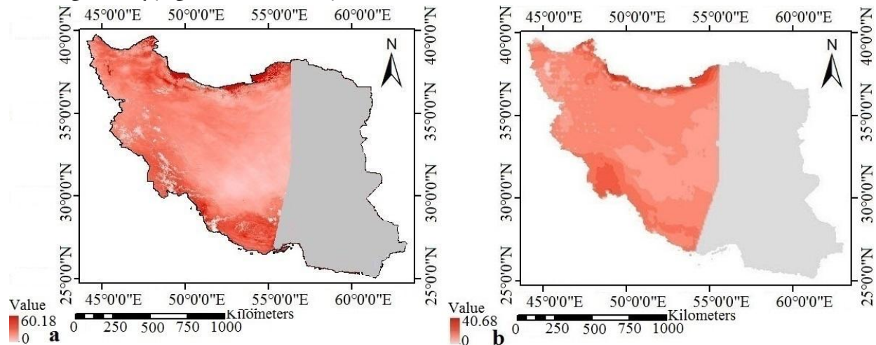
Fig. 3- The zonation map of TPW in the western part of Iran (July 12, 2015), a) MOD05 product and b) AMSR2 algorithm
