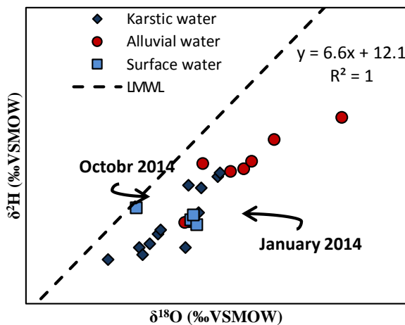
Fig. 6- Comparison of isotopic composition ( \delta^2\text{H} , \delta^{18}\text{O} ) of surface water with alluvial and karstic water
