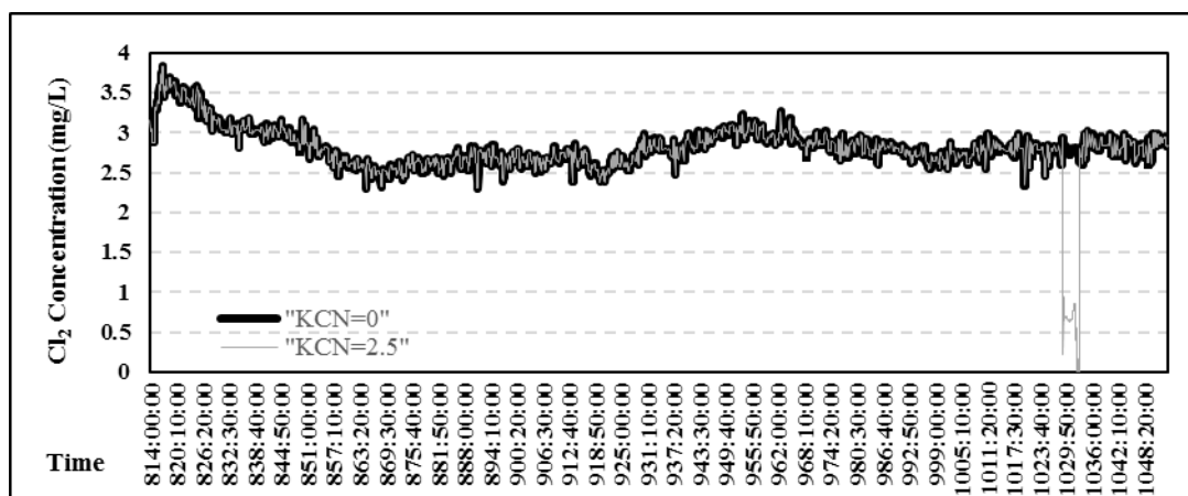
Fig. 3- Chlorine concentration at node 119 with and without KCN injection
