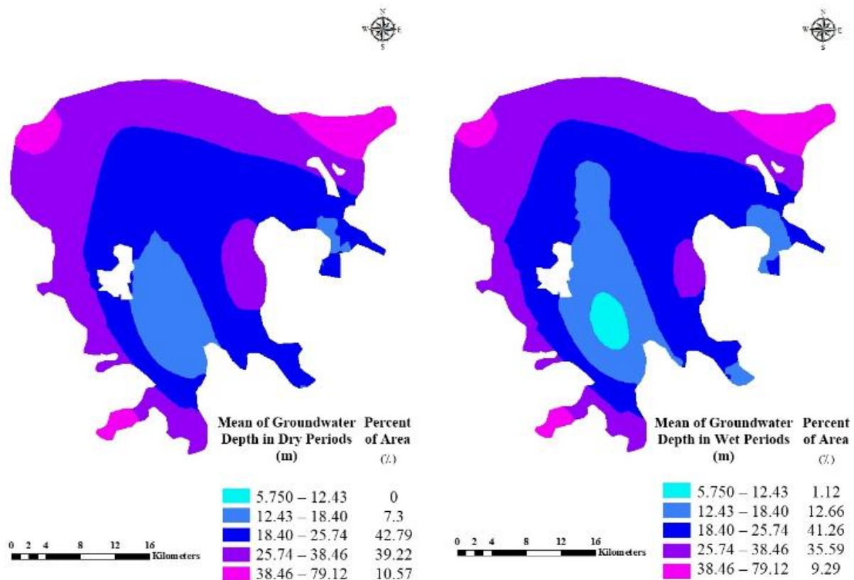
Fig. 4- The average groundwater depth in dry and wet season during 1996 to 2014
