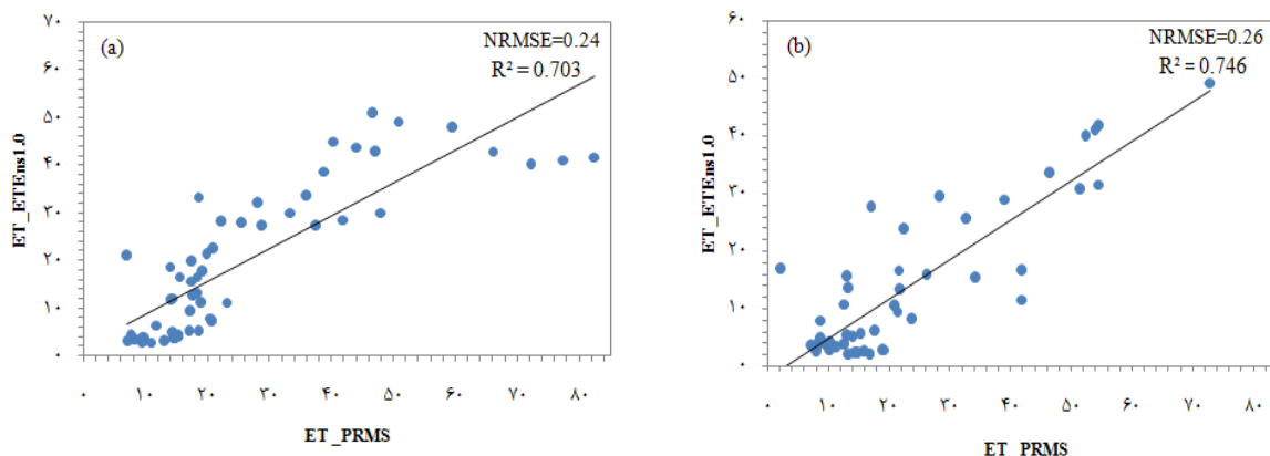
Fig. 4- Comparison between Monthly evapotranspiration in PRMS and ETEns1.0 in (a) calibration (b) validation
