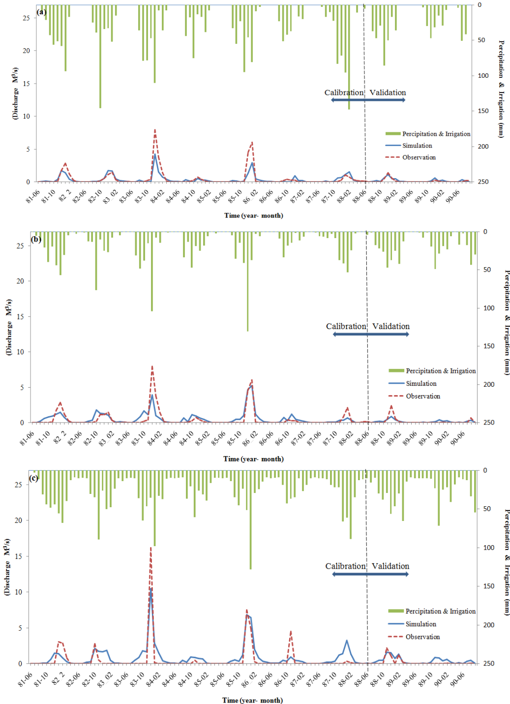
Fig. 5- Observed and simulated runoff and sum of precipitation and irrigation in upstream of (a) AndarAb, (b) Kharve and (c) Hossein Abad stations
