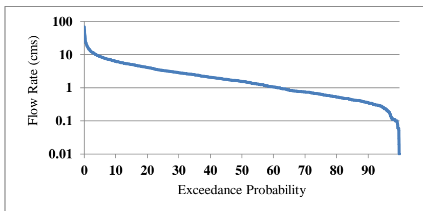
Fig. 4- Flow Duration Curve of Kazemrud River
