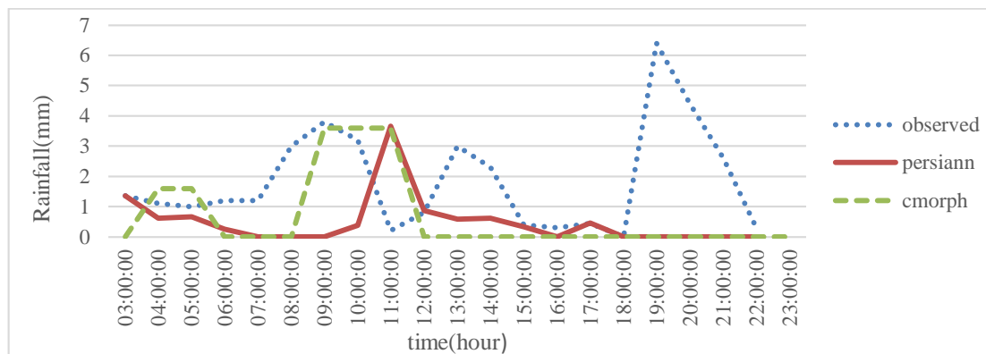
Fig. 5- Comparison of PERSIANN and CMORPH result against Boushigan gauge data (rainfall event 06/01/2014)
