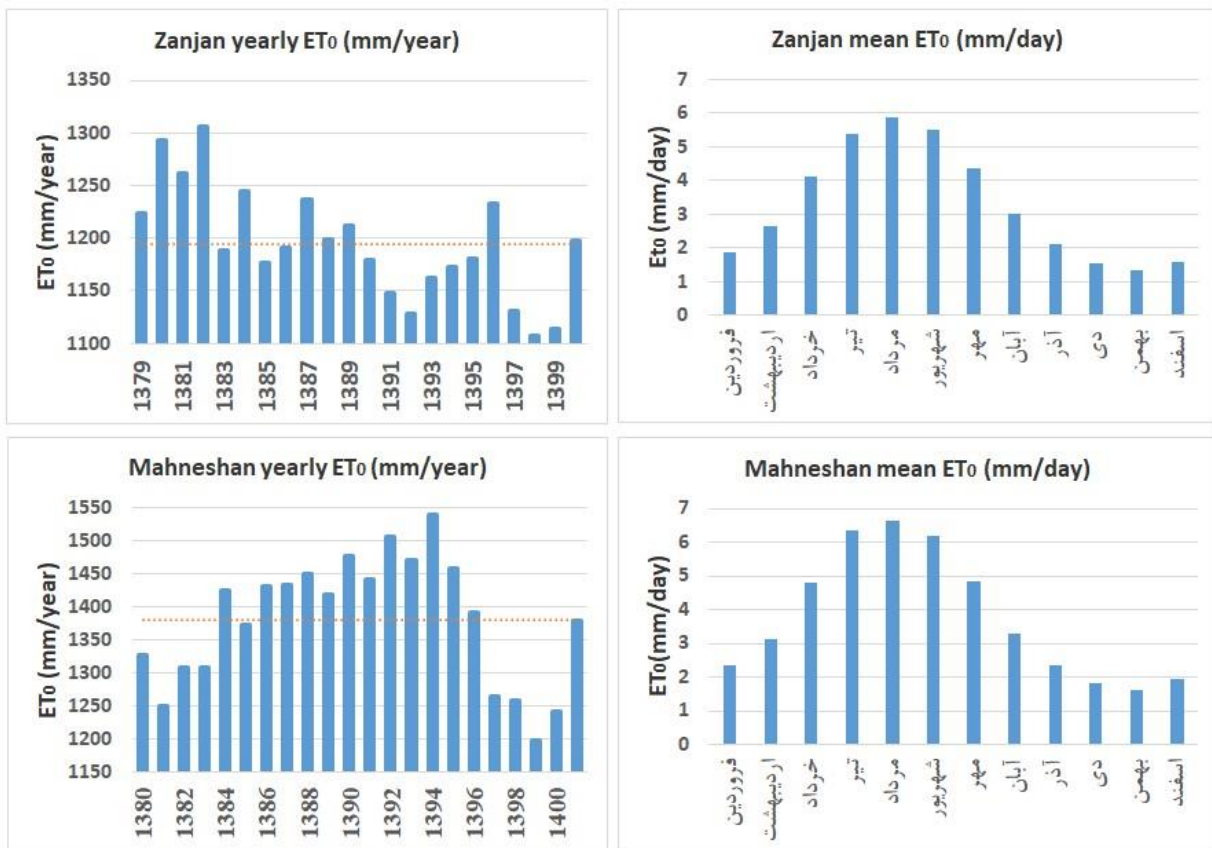
Fig. 3- plots of reference evapotranspiration time series in annual scale (left) and monthly distribution pattern (right) at the two stations Zanjan (up row) and Mahneshan (bottom row) in the time period (1379-1400)
