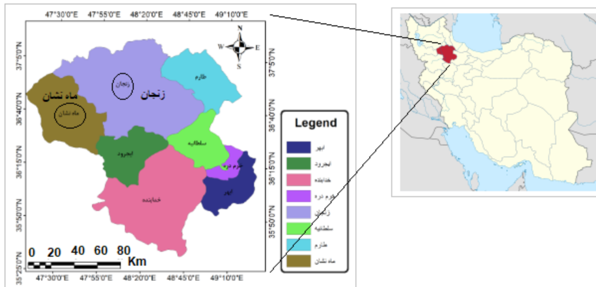
Fig. 1- Geographical location of the Zanzan province as the study area
