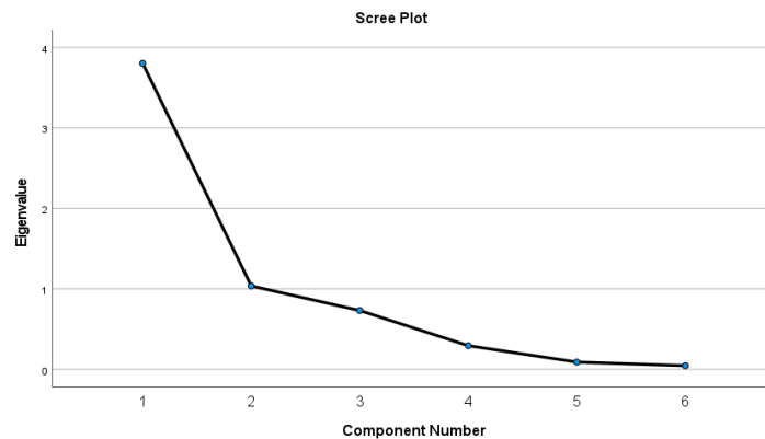
Fig. 4 Screeplot resulting from decomposition into main components in Zanjan station
