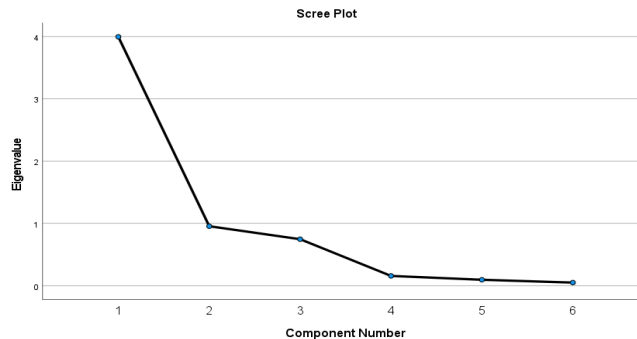
Fig. 6- Screeplot resulting from decomposition into main components at Mahneshan station
