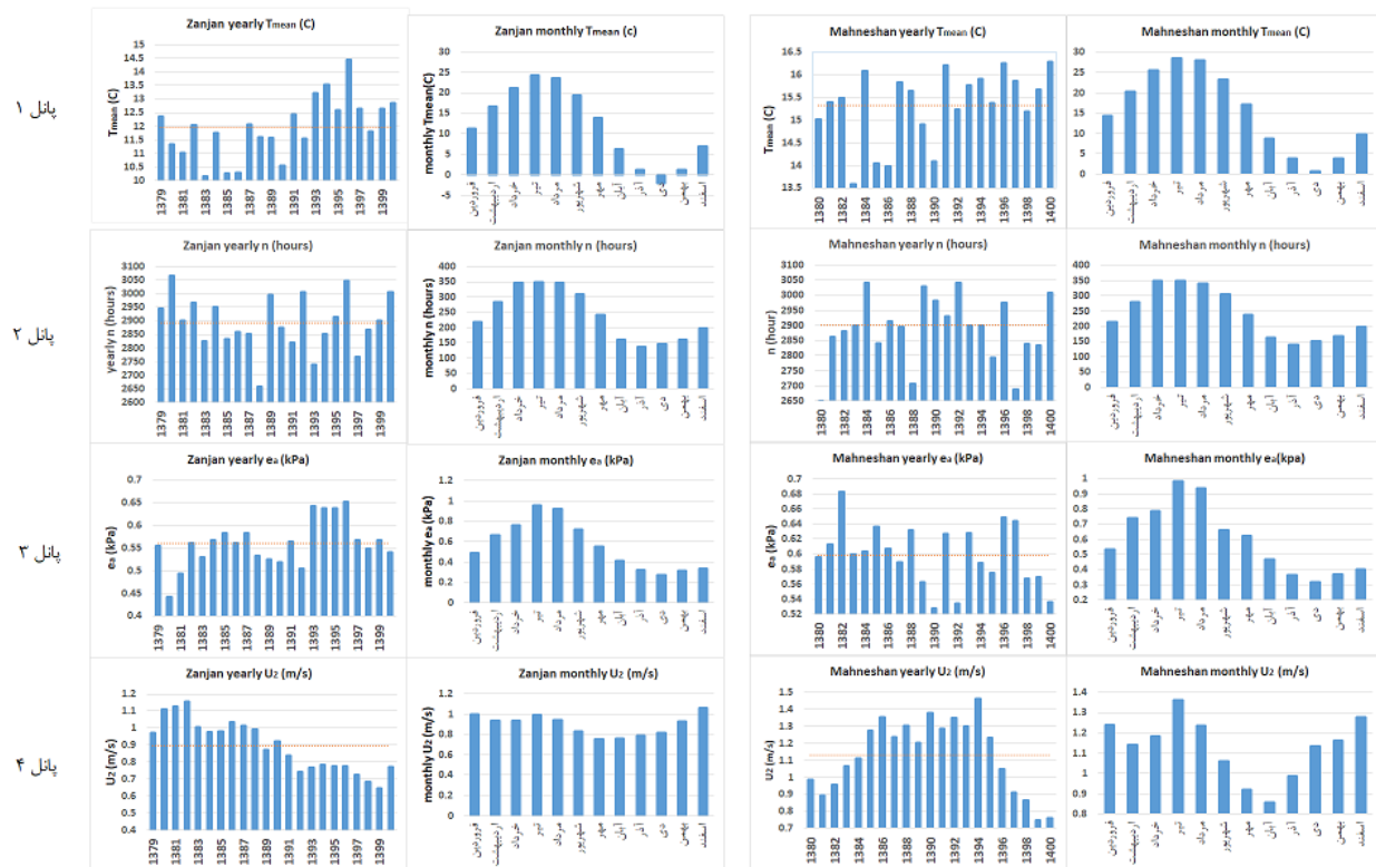
Fig. 2- Plots of climatic variables in the stations Zanjan and Mahneshan (1379-1400)
