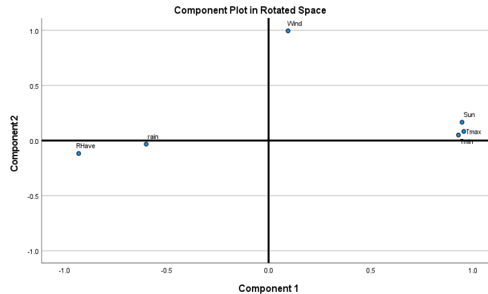
Fig. 7- Chart of the coefficients of the first and second factors at Mahneshan station after rotation of axes
