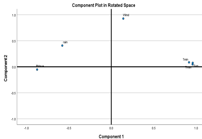
Fig. 5- Chart of the coefficients of the first and second factors at Zanjan station after rotation of axes
