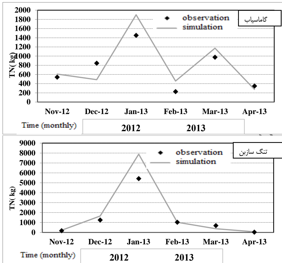
Fig. 6- Comparison of simulated and observed total nitrogen in monitoring stations; Calibration period 2012-2013
