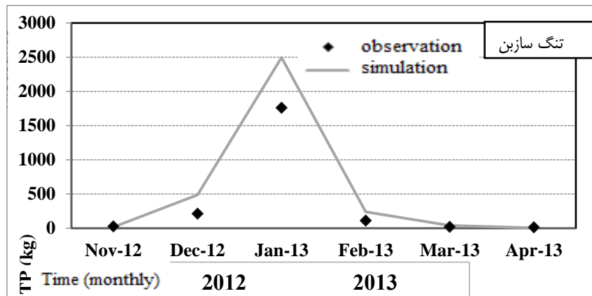
Fig. 7- Comparison of simulated and observed total phosphorus in monitoring stations; Calibration period 2012-2013
