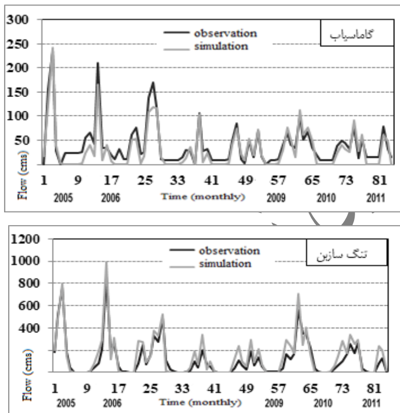
Fig. 4- Comparison of simulated and observed monthly discharge in hydrometric stations; Calibration period 2005-2011
